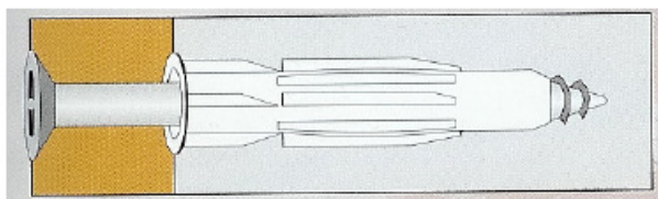
Veilige verankering in cellenbeton
